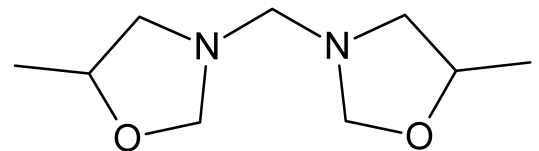
3,3'-Methylenbis[5-methyloxazolidin] (MBO)
